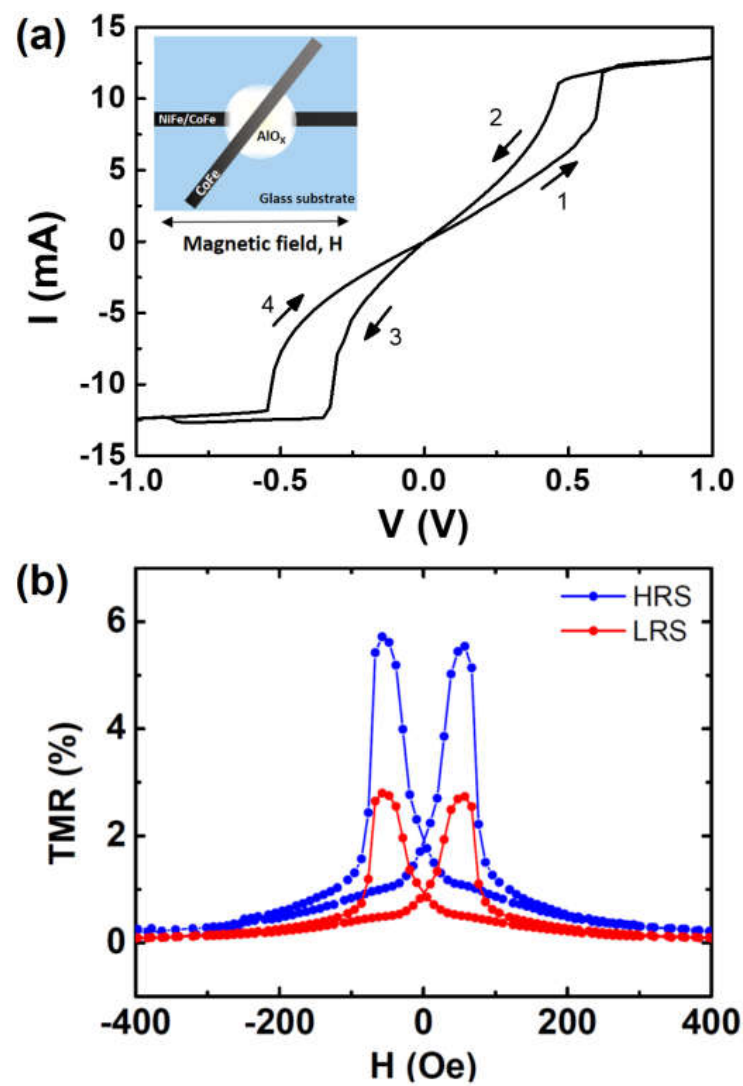
Figure 1. (a) Current–voltage ( I – V ) curve of a NiFe/CoFe/ \text{AlO}_x /CoFe RS memory device with arrows indicating the directions of the voltage sweep. Note that the threshold setting and resetting voltage was about 0.6 V and -0.6 V, respectively. (b) The room-temperature TMR as a function of the magnetic field measured at 2 mV for HRS and LRS, respectively. The inset shows the scheme of the device structure.
