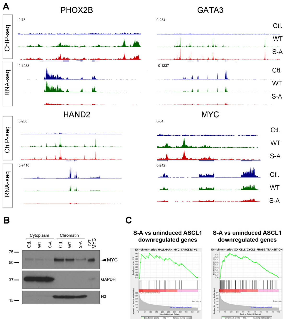
Fig 2. Dephosphorylated ASCL1 suppresses the oncogenic core regulatory circuit of NB cells (A) ChIPseq and RNAseq tracks of PHOX2B , GATA3 , HAND2 and MYC in NB cells, either uninduced (Ctl) or 24 hours post-induction of WT and S-A ASCL1. ChipSeq n=8 in 4 biological replicates, RNAseq n=10 in 5 biological replicates. (B) Western blotting for MYC within the cytoplasm and chromatin fractions either uninduced (Ctl) or 24 hours post-induction of WT and S-A ASCL1, GAPDH (control for cytoplasmic fractionation) and histone H3 (control for chromatin fractionation).
