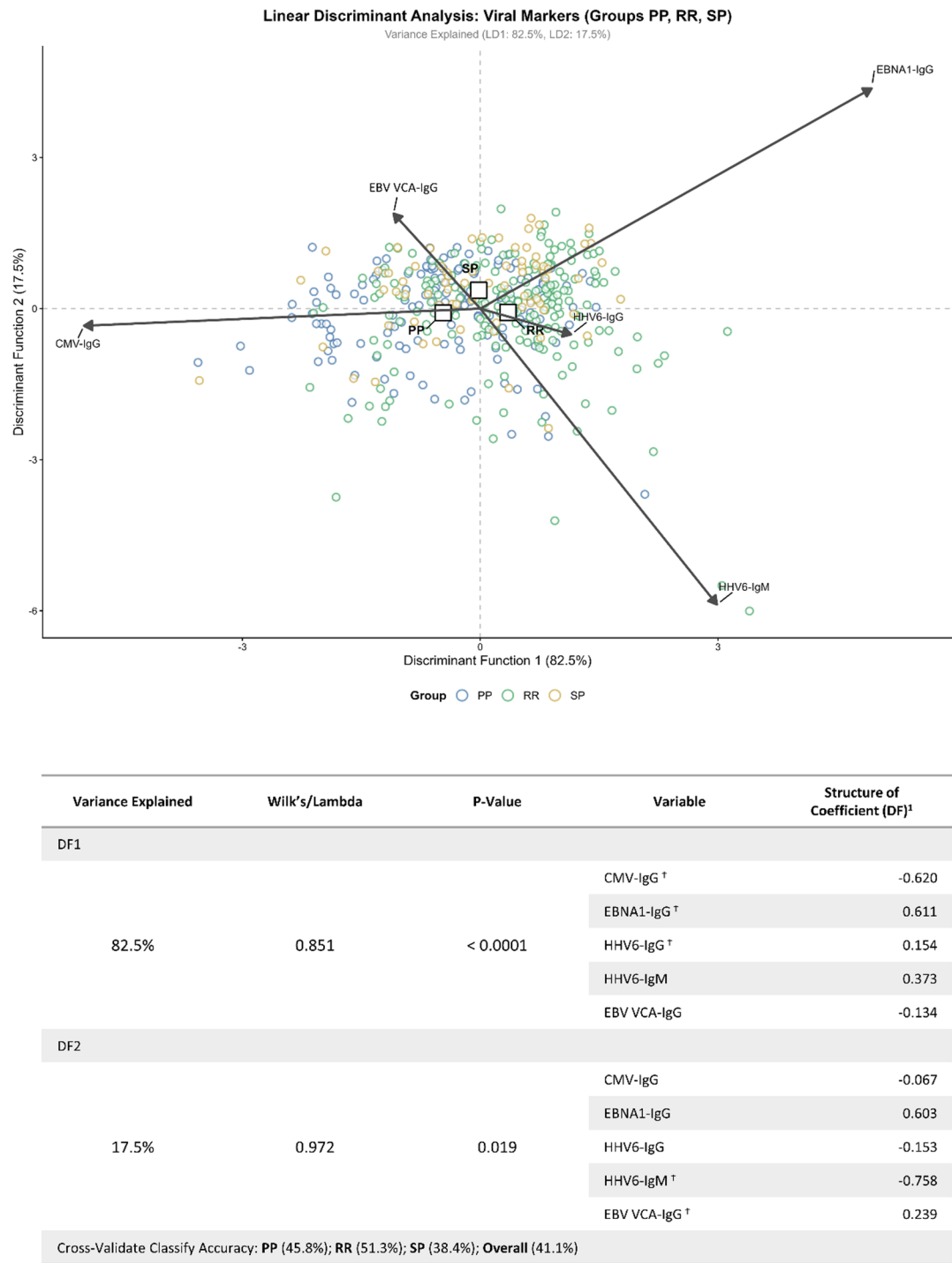
Fig. 2. A discriminant analysis biplot with vectors representing EBNA-1 IgG, EBV VCA IgG, CMV IgG, HHV-6 A/B IgG and HHV-6 A/B IgM. Points close together are similar observations, and the angles between variable arrows indicate their correlation (acute for positive, right for 0, obtuse for negative).
