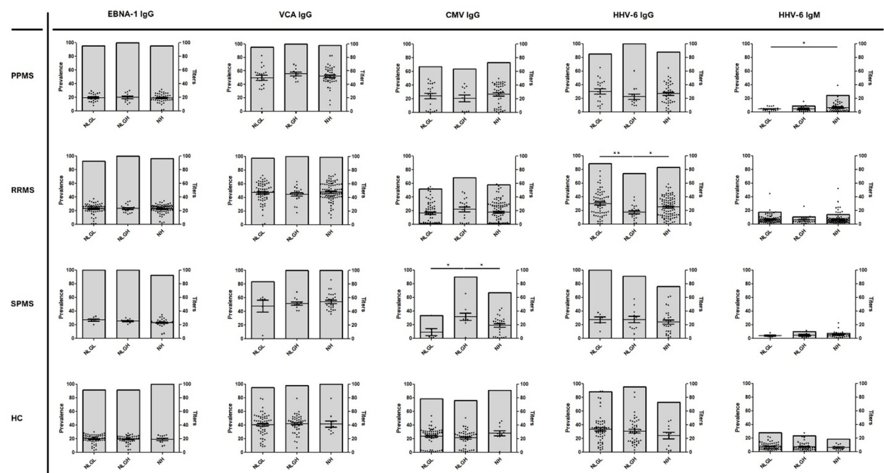
Fig. 3. EBNA-1, VCA, CMV and HHV-6 A/B IgG and IgM prevalences and titers in PPMS, RRMS, SPMS and HC cohorts after stratification by sNfL and sGFAP levels: NLGL (low sNfL < 10 pg/ml and low sGFAP < median value), NLGH (low sNfL < 10 pg/ml and high sGFAP > median value), and NH (high sNfL > 10 pg/ml) at different levels of sGFAP. Height of the grey columns show the viral prevalences. Median and interquartile range (P25 and P75) for viral titers are also shown. * ( p < 0.05 ); ** ( p < 0.005 ); *** ( p < 0.0005 ).
