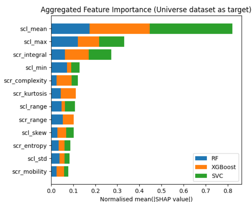
Figure A1. Aggregated SHAP-based feature importance for the UNIVERSE dataset as target domain. Bars represent the normalised mean absolute SHAP values, stacked to show the relative contribution of the RF, XGBoost, and SVC classifiers.
