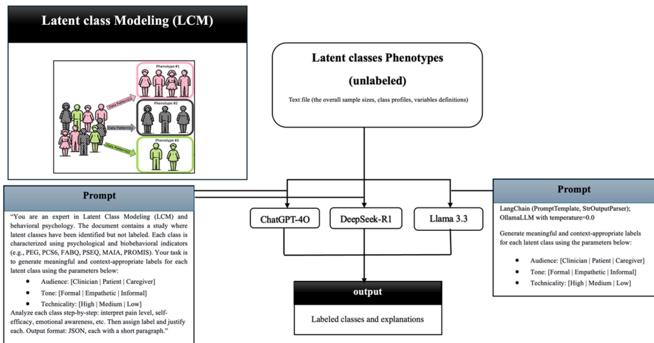
Figure 1 Schematic representation of the LLMs model.
